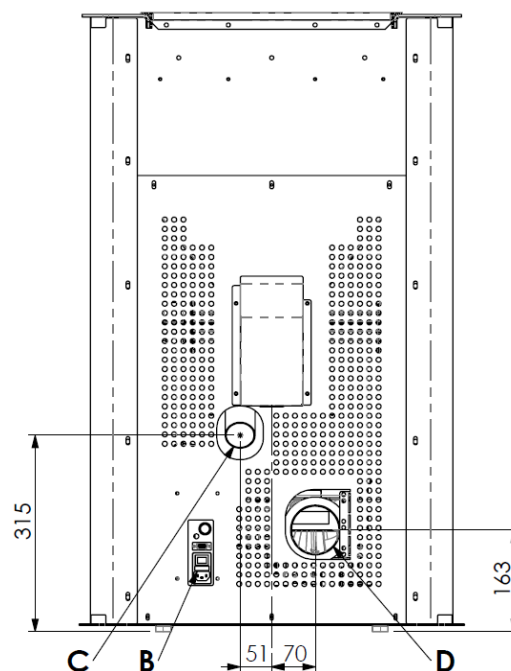
AURORA pellet stove dimensions
